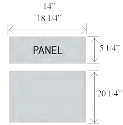
Opening Dimensions
