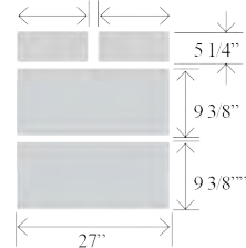
Opening dimensions
